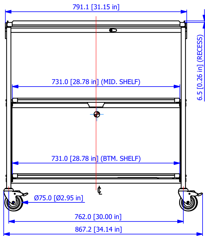
FRONT
