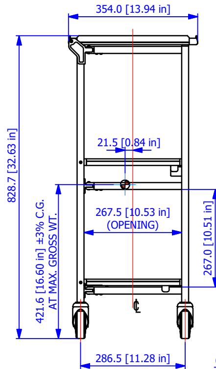
SIDE
