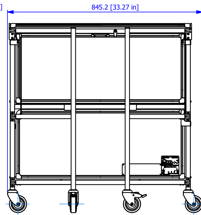
FOLDED VIEW
