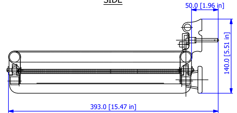
FOLDED VIEW
